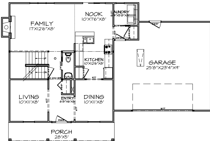
FIRST FLOOR PLAN A-4
